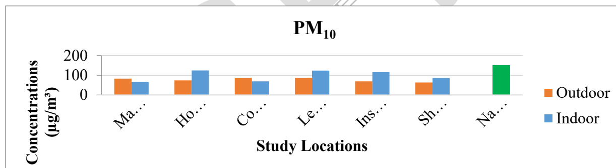
Figure 1: Illustration of PM 10 in the Study Locations
